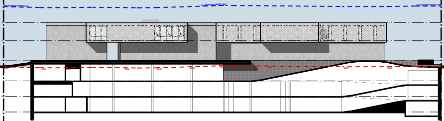
NORTH ELEVATION | McARTHUR STREET 1:500
