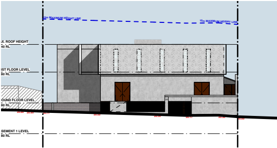
NORTH ELEVATION | McARTHUR STREET 1:500
